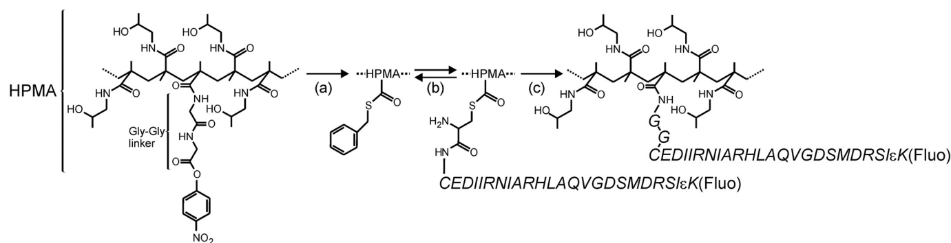
Scheme 1. Synthesis of a HPMA-BH3 conjugate. a, DMSO (anhydrous), benzylmercaptane; b, DMSO (anhydrous), thiophenol; c, DMSO, thiophenol, phosphate buffer (100 mM), guanidiniumchloride (6 M, pH 7.5). Amino acids are represented in single-letter code and printed in italics.
