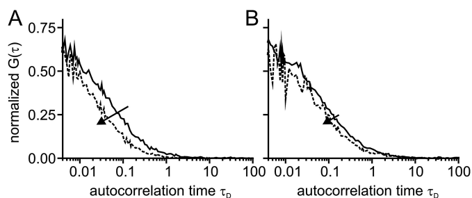
Fig. 7. Proteolytic stability of HPMA-BH3 and the free BH3 peptide in living Jurkat E6.1 cells. The conjugate/peptide was electroporated into cells. After incubation, cell lysate was generated and measured by FCS. Whereas the diffusion time \tau_D of the free BH3 peptide decreased significantly upon incubation in cells (A), the \tau_D of the HPMA-BH3 decreased only slightly (B). The shifts in diffusional autocorrelation times between the intact conjugate or peptide (solid lines) and the incubated samples (dashed lines) are indicated by arrows.
