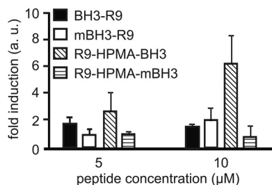
Fig. 8. Apoptosis induction by R9-HPMA-BH3. Jurkat cells were incubated with conjugates for 6 h at 37°C. Titration of cells with HPMA-R9 conjugates and peptide-R9 conjugates and determination of caspase-3-activity. Concentrations of the polymer conjugates in the medium were adjusted to the same concentration with respect to the functional peptide. For the HPMA conjugates and the free peptides, the normalized mean and mean error of two and four independent experiments is shown.
