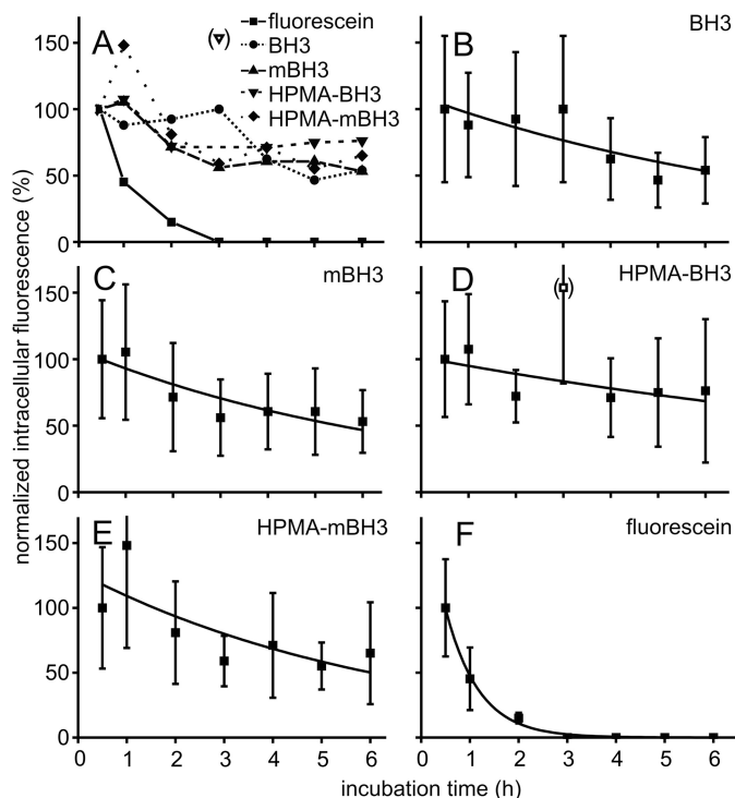
Fig. 4. Analysis of release kinetics. The confocal images generated by laser scanning microscopy (Fig. 3) were analyzed by quantitative image analysis. A, superposition of all curves (the intensity at the beginning of the experiment was set to 100%). B, free BH3 peptide. C, free mBH3 peptide. D, HPMA-BH3 conjugate. E, HPMA-mBH3 conjugate. F, fluorescein. The data were fitted with a first-order exponential decay.
