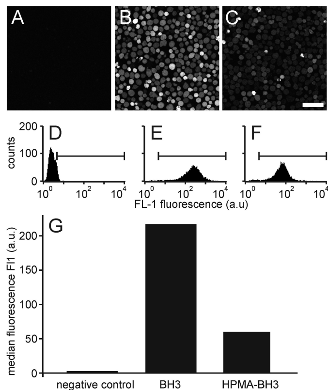
Fig. 2. Electroporation efficiency of free peptides and HPMA-peptide conjugates. Jurkat E6.1 cells were electroporated with medium (A) 30 \mu\text{M} free BH3 peptide (B), or HPMA-BH3 (C). The concentration of conjugate relates to the number of peptide moieties. Thereafter, the living cells were washed with medium and observed by confocal laser-scanning microscopy 1 h after electroporation (A–C); scale bar, 50 \mu\text{m} . D–F, corresponding flow cytometry histograms; G, medians of intracellular fluorescein intensities.
