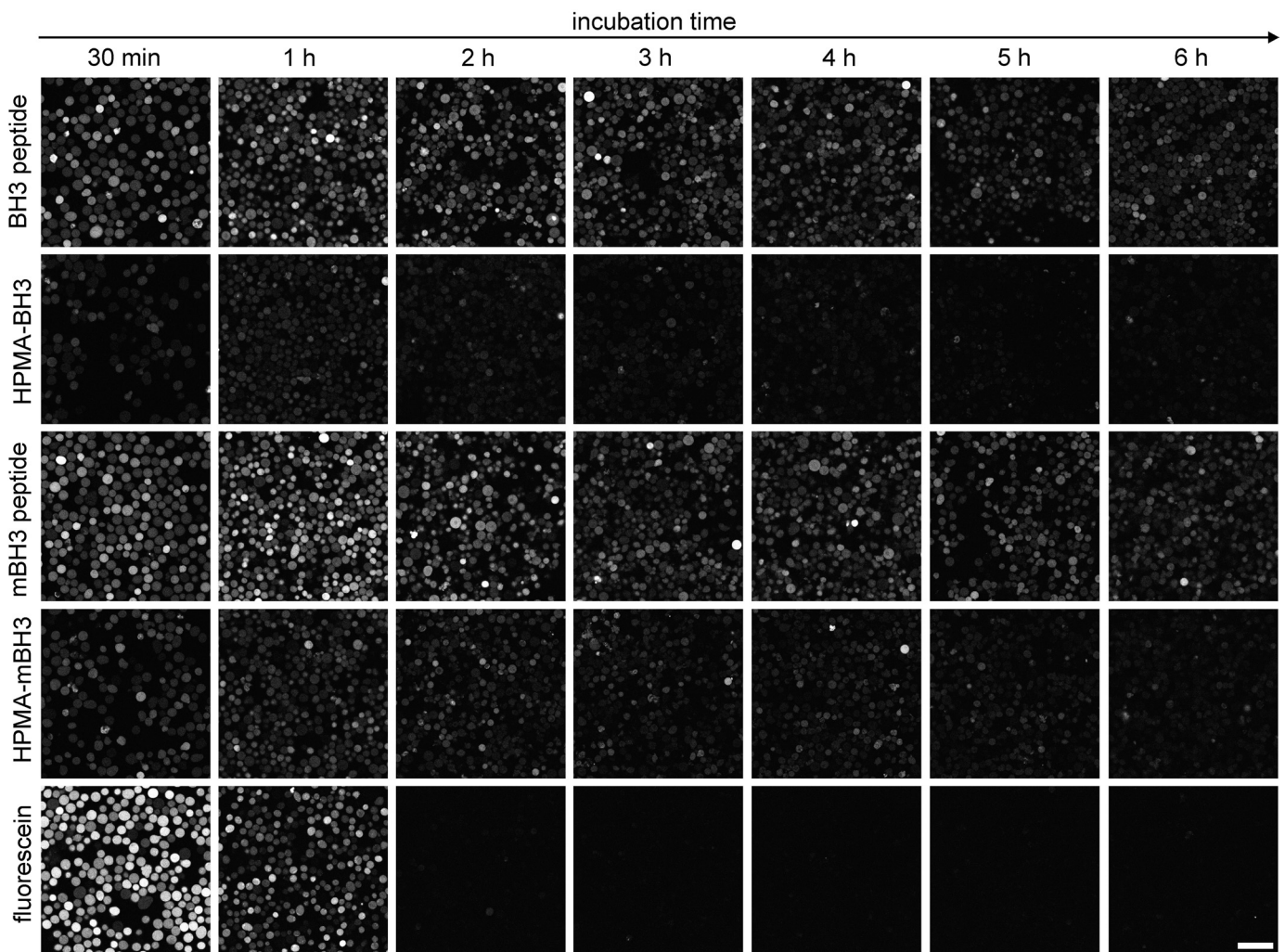
Fig. 3. Release of cellular fluorescence after electroporation of free peptides and HPMA-peptide conjugates. Jurkat E6.1 cells were electroporated with 30 \mu M free peptides and HPMA-peptide conjugates or fluorescein. The concentration of conjugate relates to the number of peptide moieties. Thereafter, the cells were washed twice with medium, seeded into an eight-well chambered coverglass, and incubated at 37°C. In certain time intervals, confocal images were taken by laser scanning microscopy. Scale bar, 50 \mu m.
