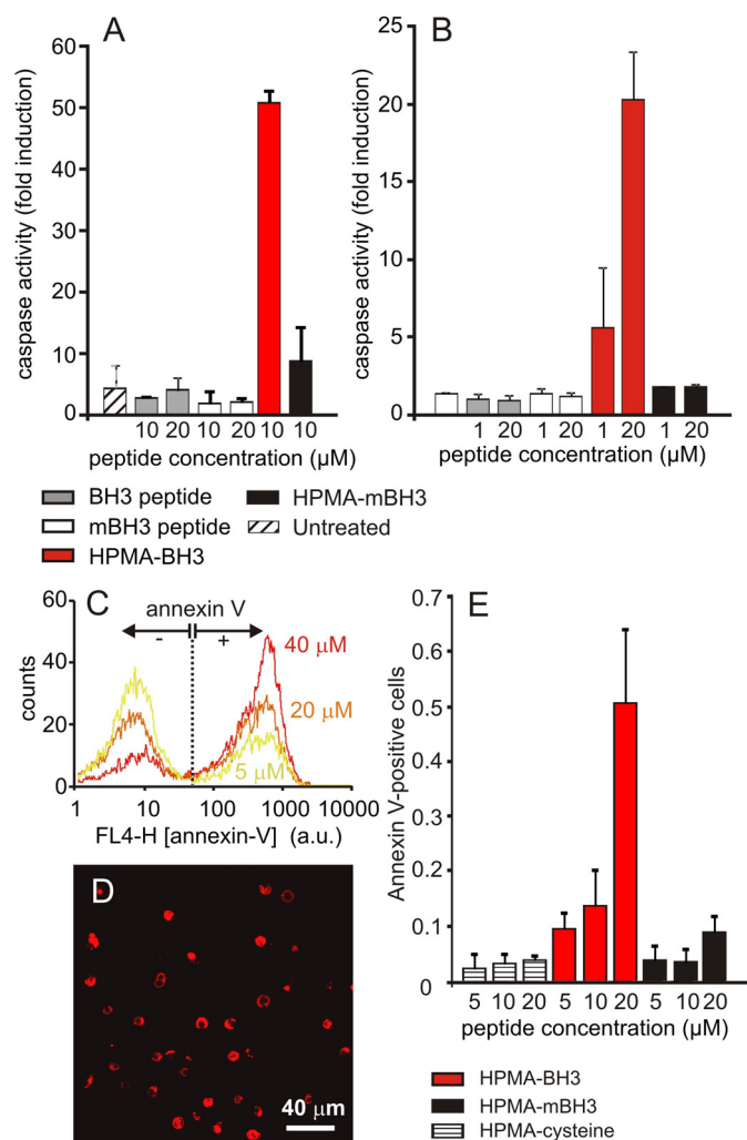
Fig. 1. Apoptosis induction by HPMA-peptide conjugates and free peptides. Jurkat or HeLa cells were electroporated with the free apoptosis-inducing BH3 peptide, the mutated mBH3 peptide or the respective polymer-conjugated peptides HPMA-BH3 and HPMA-mBH3 at the indicated concentrations. A and B, determination of caspase-3 activity in Jurkat cells (A) and HeLa cells (B) lysed 6 h after electroporation with free peptides and HPMA-peptide conjugates. Error bars indicate the S.D. from two independent experiments. The concentrations relate to the number of bioactive peptides. C to E, apoptosis detection by Annexin V staining. After electroporation, the cells were washed and incubated in fetal calf serum-containing medium for 20 h with HPMA-peptide conjugates. Thereafter, cells were stained with Alexa Fluor 647-labeled Annexin V. C, flow cytometry histograms of Jurkat cells electroporated with various concentrations of HPMA-BH3 and stained with Alexa Fluor 647-labeled annexin-V. D, microscopy image of Annexin-V-stained cells, electroporated with 40 \mu\text{M} HPMA-BH3, 20 h after incubation. E, Annexin-V positive cells represented as the normalized fraction of Annexin-V-positive cells for the indicated concentrations of the HPMA-peptide constructs. The error bar shows the S.E. of three independent experiments.
