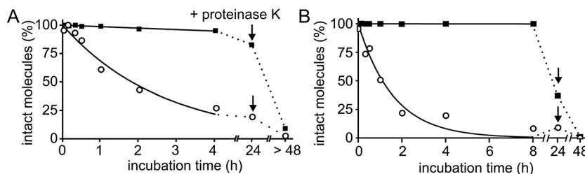
Fig. 6. Proteolytic stability of HPMA-BH3 and the free BH3 peptide in crude cell lysates of HeLa (A) and Jurkat E6.1 (B) cells. Cell lysate was generated by lysis of cells in Triton X-100. The cell lysate was mixed with 2 \mu M HPMA-BH3 conjugate or free BH3 peptide and the samples were incubated at 37°C. The concentration is related to the number of peptide moieties. After certain time points, samples were extracted and frozen. After 24 h, proteinase K was added to the samples to confirm the general sensitivity to proteases. The fractions of intact conjugate (■) and peptide (○) were determined by fluorescence correlation spectroscopy and derived from two-component fits of the autocorrelation functions. Half-lives were derived from first-order exponential fits. Shown are the results of a representative experiment for either cell line.
